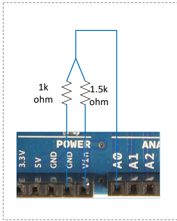
Low Voltage Status Indication (voltage divider)
