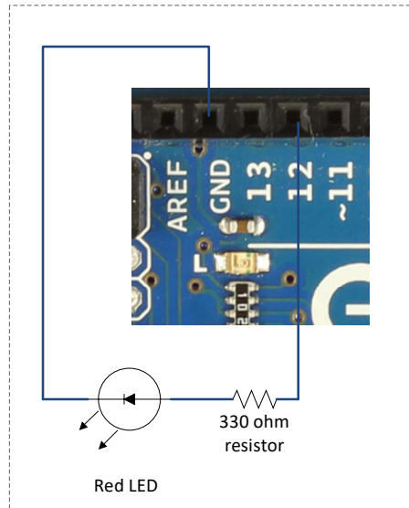
Low Voltage Status Indicator (Red LED)
